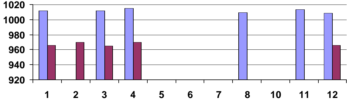
Mean Barometric Pressure (mb)
